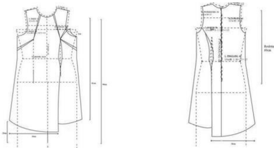
Gambar 4 (Pola belakang dress busana 1)
